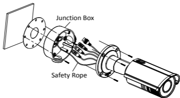
Figure 2-14 Mounting with a Junction Box
