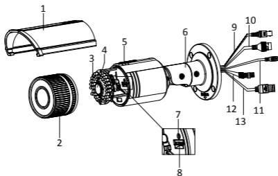
Figure 1-4 Overview of Type III Camera (1)
