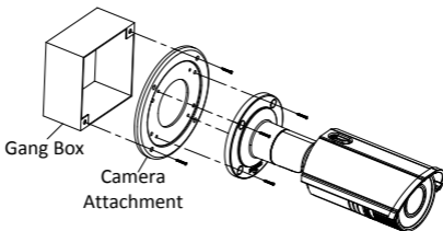
Figure 2-15 Mounting with a Gang Box
