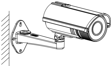
Figure 2-6 Install the Camera to the Bracket
